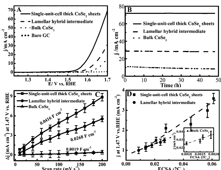
Figure 4. Electrochemical properties for the single-unit-cell thick CoSe 2 sheets, lamellar hybrid CoSe 2 -DETA intermediate, and bulk CoSe 2 : A) polarization curves; B) i - t curve at 1.7 V versus reversible hydrogen electrode (RHE); C) the differences in current density variation ( \Delta j = j_s - j_c ) at a potential of 1.47 V plotted against scan rate fitted to a linear regression enables the estimation of C_{dl} ; D) current density at 1.47 V versus RHE plotted against ECSA for various materials at different loadings.
